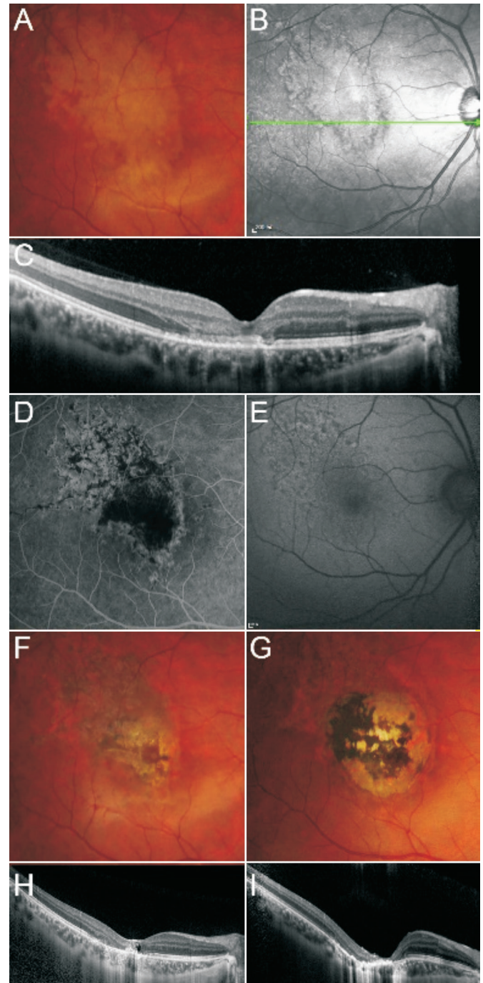
Figure 3 Case 10 A: Fundus photography at first visit shows yellow hypopigmented geographic lesion at macula. IR images (B) and OCT (C) at first visit. Hyperreflective lesion is well visualized and the margin of the lesion is delineated sharply with hyporefective line in FAF. On OCT, thinning in the outer nuclear layer and disruption of photoreceptor layers are observed. A hyperreflective band continuous with external limiting membrane is detected. Fundus FA (D) 1mo after first visit, showing tissue defect. FAF image (E) and fundus photography (F) at 2mo shows central dark pigmentation and RPE atrophy. H: OCT at 2mo shows outer retinal disruption, hyperreflective dots, and cysts in the fovea. G: Fundus photography after 1y shows central dark pigmentation and surrounding circular chorioretinal atrophy. I: OCT shows progression of outer retinal layer thinning. FCE and choroidal thinning have developed and the choroidal lesion corresponds to the round atrophic lesion seen in fundus photography.
