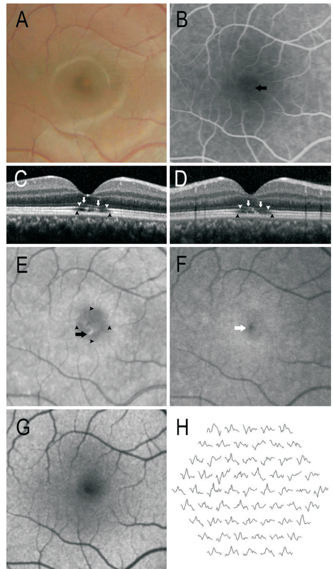
Figure 1 Results of ophthalmologic examination of a representative case (Case 7) who presented with a visual acuity of 20/200
