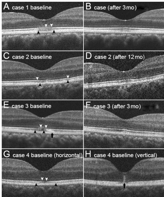
Figure 4 SD-OCT images of cases that presented with photoreceptor layer blurring with relatively preserved EZ (Group 1) Despite EZ blurring, EZ band is dimly visible in all cases. B, D, and F are follow-up images of A, C, and E images. Follow-up images of B, D, and F were taken at 3, 12, and 3mo, respectively. White arrowheads: EZ defect area; Black arrowheads: IZ defect. EZ and IZ blurring and defects show improvement in the follow-up images. The black arrows (E) indicate abnormal hyperreflectivity at the photoreceptor layer. This hyperreflectivity decreased during the follow-up. G and H are the initial OCT images (horizontal and vertical scans) of Case 4 because consecutive photo was not obtained. Central hyperreflective columnar structure is observed with surrounding hyporefective area (black arrow).
