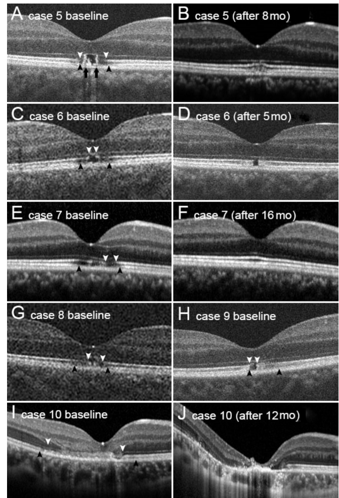
Figure 5 SD-OCT images of cases that presented with discrete photoreceptor layer defects involving EZ (Group 2) A, C, E, G, H, I: The baseline images show severe outer retinal defects and surrounding hyporefective areas with discontinuation of EZ. B, D, F, J: The follow-up images of Cases 5, 6, 7, and 10 taken after 8, 5, 16, and 12mo, respectively. White arrowheads: EZ defects; Black arrowheads: IZ defects. The photoreceptor disruption recovered either partly or completely, except in Case 10. Black arrows in image A indicate hyperreflective columnar structure in the photoreceptor layer. I: Outer plexiform layer is thickened but its margin is indistinct. Hyperreflective band continuous with external limiting membrane is visible between white arrowheads. J: Outer nuclear layer and outer plexiform layer are invisible; instead hyperreflective material is detected at foveola. Choroidal curvature has become steeper after a year.
