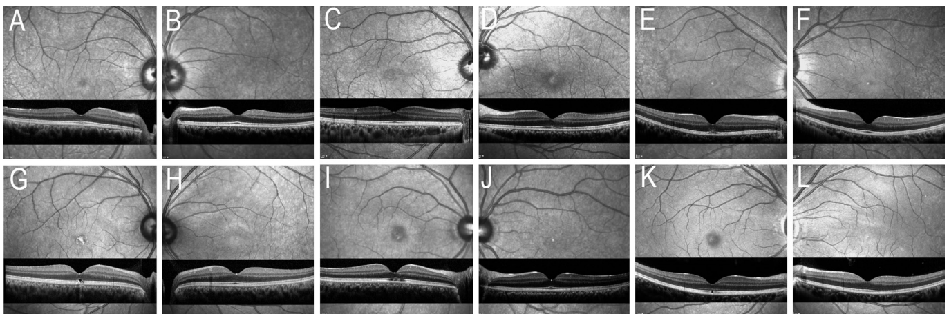
Figure 7 IR images (820 nm) of Case 1 (A and B), Case 3 (C and D), Case 4 (E and F), Case 5 (G and H), Case 7 (I and J), and Case 9 (K and L) Increased reflectivity with surrounding hyporeflexive ring is observed in all cases except Case 4. Corresponding OCT images are shown under the respective IR images. A, D, E, G, I, and K are images of the involved eyes.
