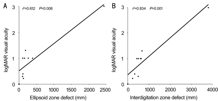
Figure 6 Correlation between size of EZ defect and logMAR visual acuity (A) and between IZ defect size and logMAR visual acuity (B) Visual acuity significantly correlated with size of EZ and IZ defect. Outliers located at the right upper corner in A and B, indicate Case 10.
