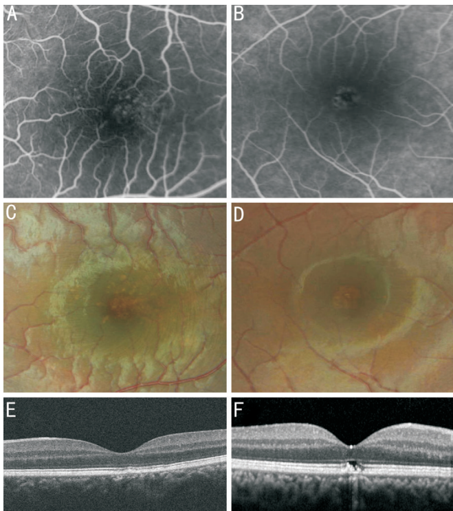
Figure 2 Fluorescein angiogram, fundus photograph, and SD-OCT A, C and E: Case 2. A speckled pattern of transmission defects on FA and corresponding pigment mottling on fundus photography are observed. The lesion corresponds to the decreased EZ and RPE reflectivity on OCT. B, D, and F: Case 5. A ring-shaped transmission defect and corresponding pigment mottling are observed. The lesion also coincides with EZ and RPE defect on OCT.
